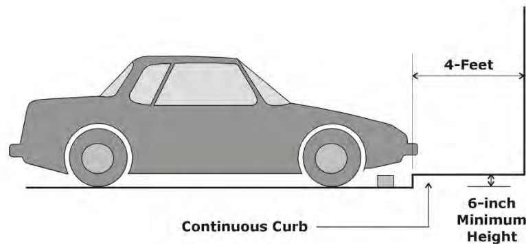
Figure 7.04-D: Continuous curbs.
